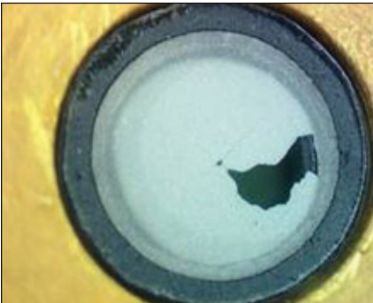
Damage caused by repeated thermal cycling to a thin substrate material spanning a large hole in an aluminum block.
