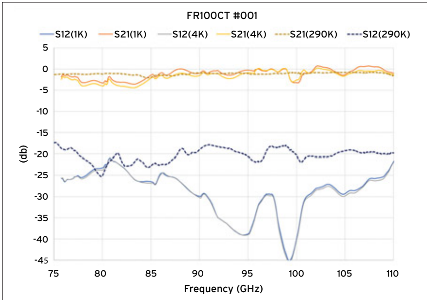
Cryogenic test results carried out at the University of Chicago at 4 K and 1 K compared with room-temperature (290 K) data. S21 shows transmission through Micro Harmonics' cryogenic isolator, while S12 represents the transmission in the reverse direction. At cryogenic temperatures, forward transmission remains high while reverse transmission decreases, demonstrating low insertion loss and high isolation. Precise measurement of the insertion loss was not possible due to calibration issues in the cryostat. The isolator insertion loss is thought to be less than 0.5 dB across the full WR-10 band.
